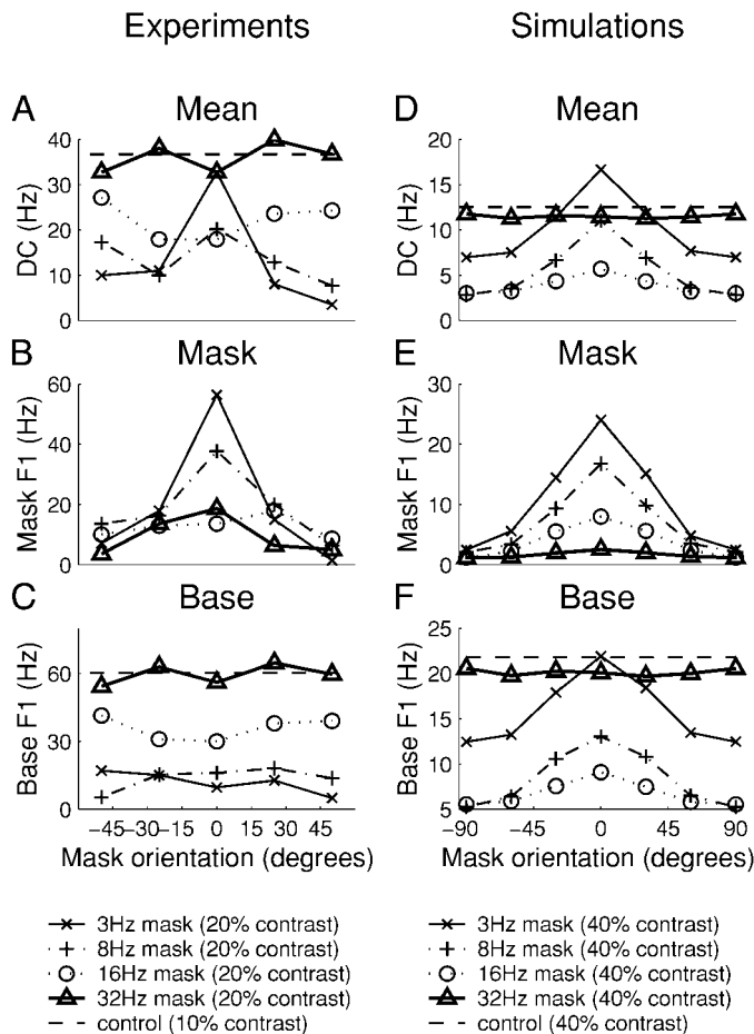
FIG. 9. Dependence of suppression on orientation and temporal frequency of mask grating, added to base grating at preferred orientation and 2 Hz. Experiments reproduced from Bonds (1989) (A–C: data for a single simple cell), and corresponding simulation results (D–F: mean response over cells with similar orientation preference). “Control” is response to base grating alone. A and D: mean (DC) spike response. B and E: F1 of the spike response at the mask temporal frequency. C and F: F1 of spike response at the base temporal frequency. In general, inhibition peaks at higher temporal frequencies in the simulations than in the experimental cell. As earlier, the simulated base response is tuned with the mask orientation, while the experimental base response is not. Simulated base current response is untuned (not shown).
