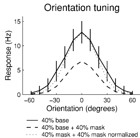
FIG. 5. Model orientation tuning curves with and without mask stimulation. —, orientation tuning curve when stimulated with a single base grating alone (mean \pm 1 SD). ---, the tuning (mean) for base grating orientation while simultaneously stimulating with a mask grating at the orientation orthogonal to the cell’s preferred orientation. \cdots , the same as --- except scaled so that the peak response matches that of the tuning curve for the base grating alone. The response reduction due to the mask grating is mainly multiplicative.
