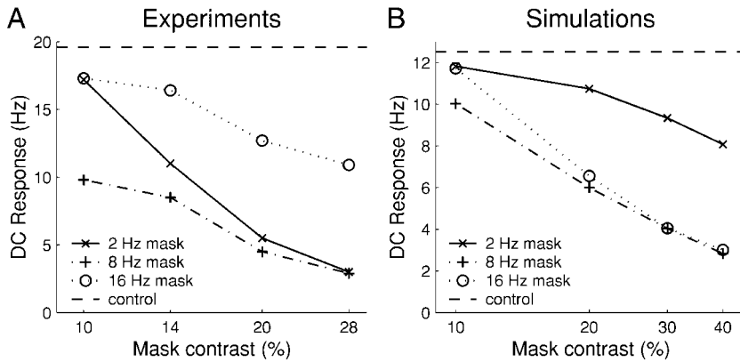
FIG. 8. Experiments reproduced from Bonds (1989) (A: data for a single simple cell), and corresponding simulation results (B: mean response over cells in simulation with similar orientation preference). Plots show mean spike response vs. mask contrast for a combination of a 2-Hz base grating at preferred orientation and a mask grating oriented at an inhibitory orientation (experiments), which we have taken to be orthogonal to the preferred (simulations). ---, response to base grating alone; —, response with 2-Hz mask; - · -, response with 8 Hz mask; · · ·, response with 16-Hz mask. The inhibitory effect of the mask grating decreases with the temporal frequency of the mask in experiments, whereas in the simulations the inhibitory effect of the mask grating is tuned toward higher temporal frequencies, thus peaking at 8 to 16 Hz, but decreasing with further increase in temporal frequency (not shown).
