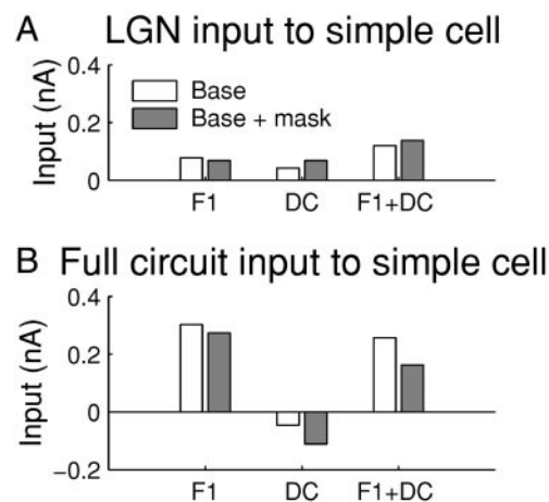
FIG. 2. F1, DC, and peak (F1 + DC) input current to a model simple cell (mean over cells with similar orientation preference) from LGN alone (A) and LGN + cortex (B) in response to stimulus grating at preferred orientation, 40% contrast alone (base); or to superposition of preferred (base) and orthogonal (mask) orientation gratings, each at 40% contrast.
