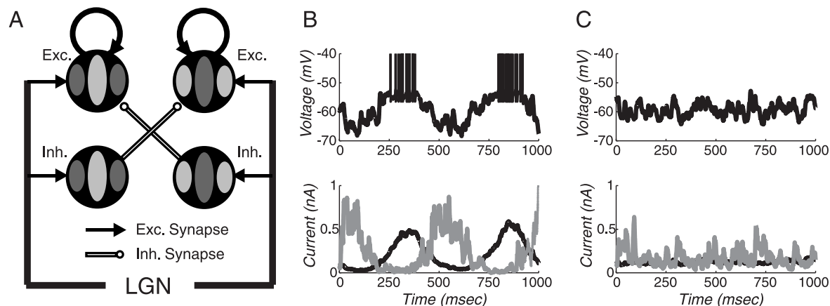
FIG. 1. A : cartoon figure of the correlation-based local cortical circuitry used in our model. Four cell pools—2 excitatory ( top ) and 2 inhibitory ( bottom ), each with 2 opposite preferred spatial phases (left vs. right)—are depicted. The 4 cell pools are at the same retinotopic position but have been separated for visibility. Light gray represents ON subfields and dark gray OFF subfields. Cells receive input from LGN and from other cortical cells preferring similar orientations. Connections are assigned probabilistically. ON center LGN inputs with centers overlying a cell's ON subregions, and OFF inputs with centers overlying OFF subregions, are likely to connect to the cell. The cells receive excitatory intracortical connections with highest probability from other excitatory cells they are most correlated with (same absolute placement of ON and OFF subfields). Inhibitory connections are received with highest probability from inhibitory interneurons they are most anti-correlated with (opposite absolute placement of ON and OFF subfields). Unlike the cartoon, the actual model includes cells of all orientations and spatial phases and spanning a range of retinotopic positions. The probabilistic sampling leads cells to receive input from other cells differing in preferred orientation by up to about 30^\circ and differing in phase from identical (excitatory connections) or opposite (inhibitory connections) by up to about 60^\circ ; the cartoon illustrates the most probable connections. The feedforward inhibition (LGN \rightarrow inhibitory cell \rightarrow excitatory cell) is stronger than the feedforward excitation (LGN \rightarrow excitatory cell). B : membrane potential ( top ) and synaptic currents ( bottom ) of a single cell as a function of time when stimulated by a drifting grating at its preferred orientation. The excitatory (black) and inhibitory (gray) synaptic currents are modulated out of phase with one another, resulting in an oscillatory membrane potential. The cell spikes during the excitatory peak of the oscillations. C : membrane potential ( top ) and synaptic currents ( bottom ) of a single cell when stimulated by a drifting grating orthogonal to its preferred orientation. There is little modulation of the synaptic current or membrane potential in time. Since the feedforward inhibition is stronger than the feedforward excitation, the membrane potential does not reach threshold.
